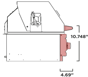
Side
